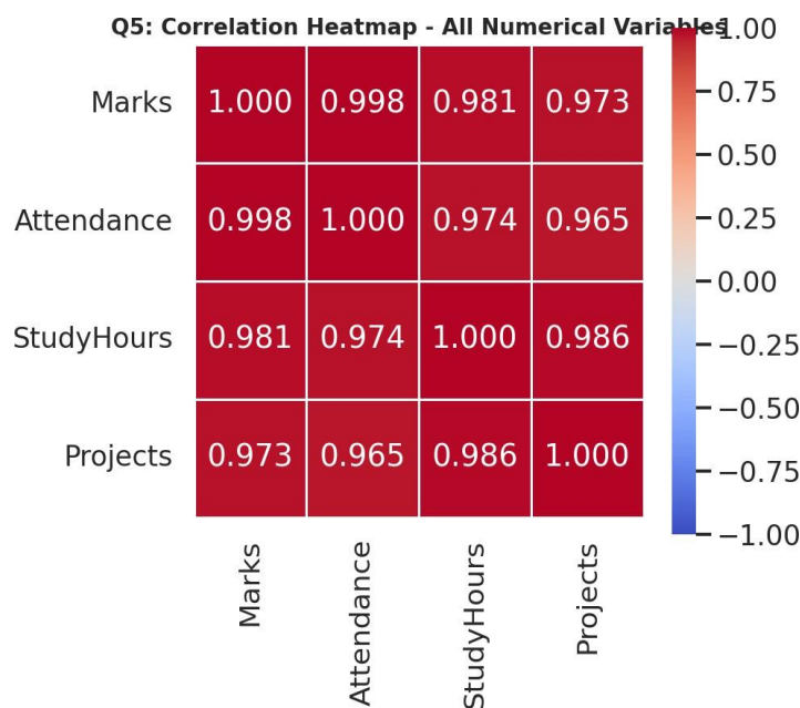
Figure 4.3 (Q5) - Correlation heatmap of all numeric variables (all pairs strongly positive, r > 0.96 ).
